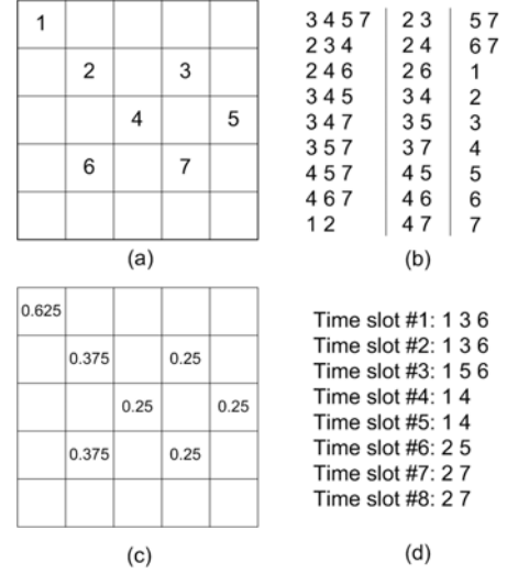
Figure 6. Obtaining the optimal sharing efficiency on gateways with IntD = 2
