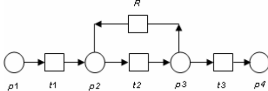
Figure 6. Circular router
