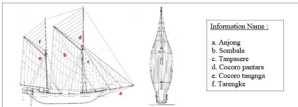
Figure 2. Blue Print Phinisi Boat Traditional with information.
