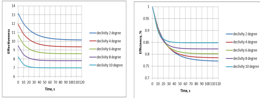
Fig. 4. Effectiveness and efficiency of fins over time, for various slope angles with the copper material, T_b = T_i = 100^\circ\text{C} , where the convection heat transfer coefficient h = 250 \text{ W/m}^2 \cdot ^\circ\text{C} .
