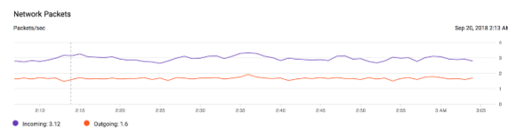
Gambar 12. Network Packet
