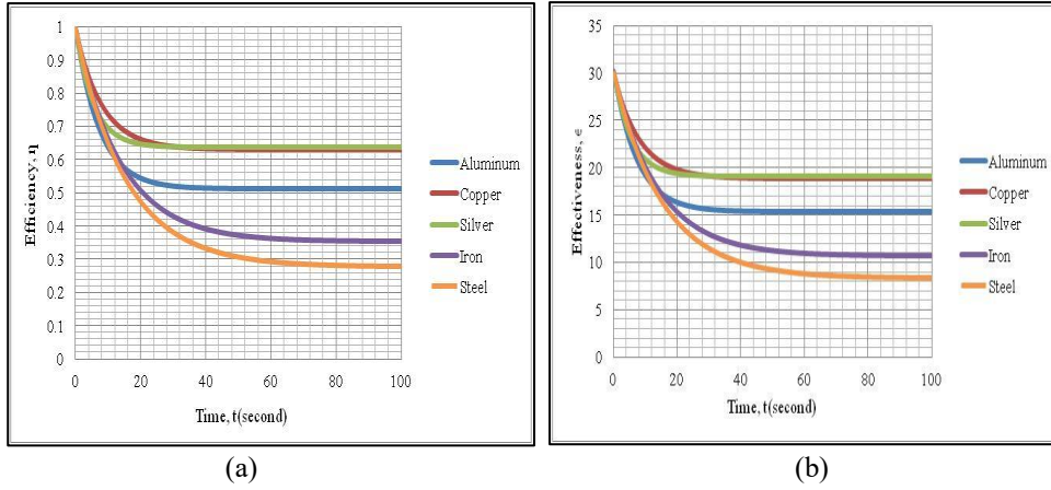
Figure 4. (a) Efficiency and (b) effectiveness of the fin with respect to time with h = 250 \text{ W/m}^2\text{°C} , \alpha = 2^\circ , T_\infty = 30^\circ\text{C} , T_i = 100^\circ\text{C} , T_b = 100^\circ\text{C}
