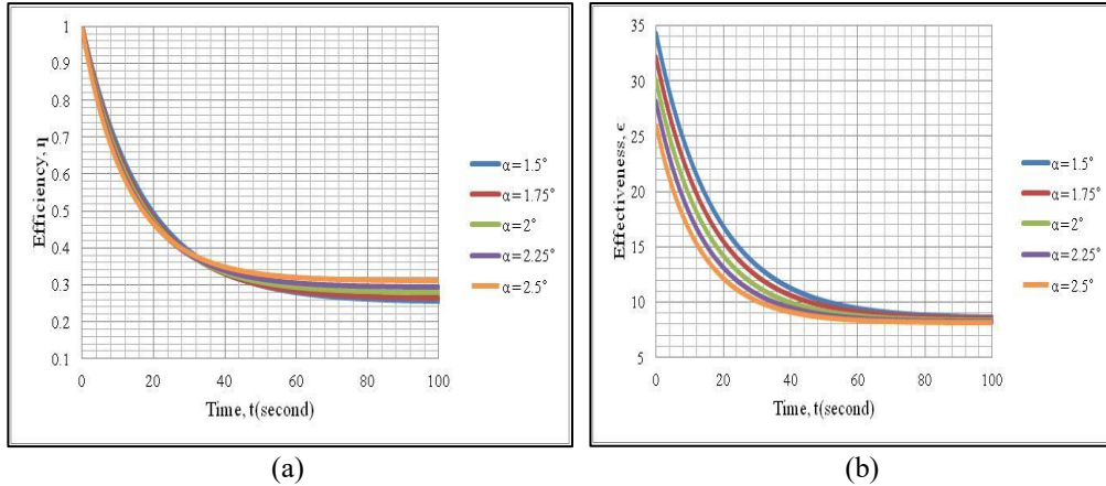
Figure 5. (a) Efficiency and (b) effectiveness of the steel fin with respect to time with h = 250 \text{ W/m}^2\text{°C} , T_\infty = 30^\circ\text{C} , T_i = 100^\circ\text{C} , T_b = 100^\circ\text{C}
