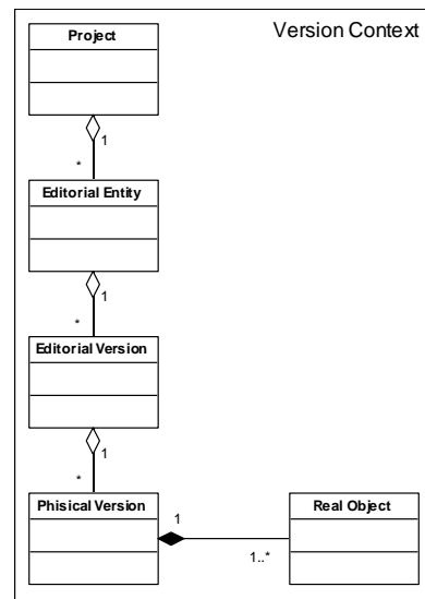
Figure 1: Version Context scheme
