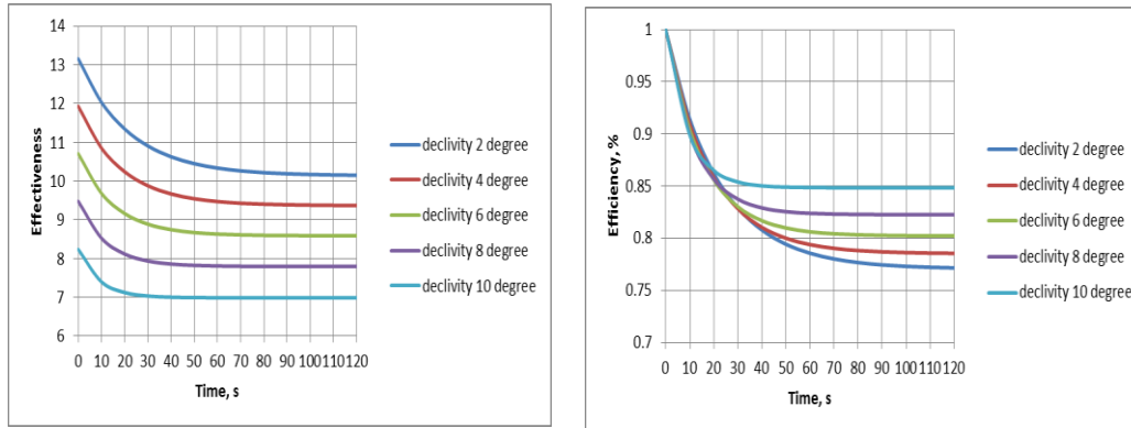
Fig. 4. Effectiveness and efficiency of fins over time, for various slope angles with the copper material, T_b=T_i=100^{\circ}\text{C} , where the convection heat transfer coefficient h=250\text{W/m}^2\text{ }^{\circ}\text{C} .
