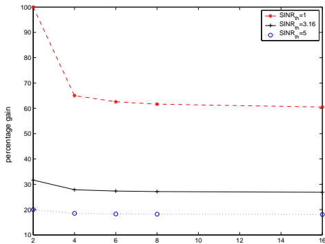
Figure 3: Percentage utility gain and network throughput gain by considering capture at different SINR_{th} .
