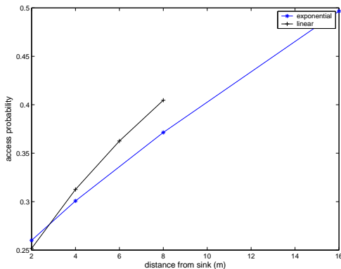
Figure 4: Access probability for linear and exponential topology
