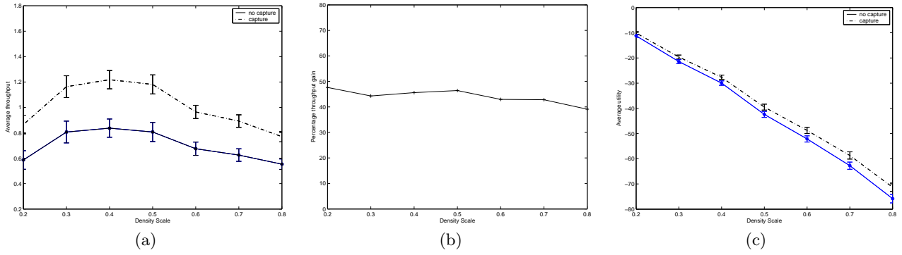
Figure 6: At SINR_{th} = 3.16 , (a) Network throughput (b) Percentage throughput gain (c) Network utility at different density scales
