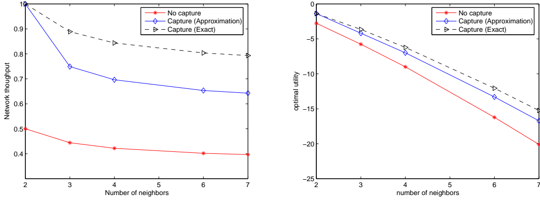
Figure 2: At SINR_{th} = 1 Network throughput and Network utility for circular topology
