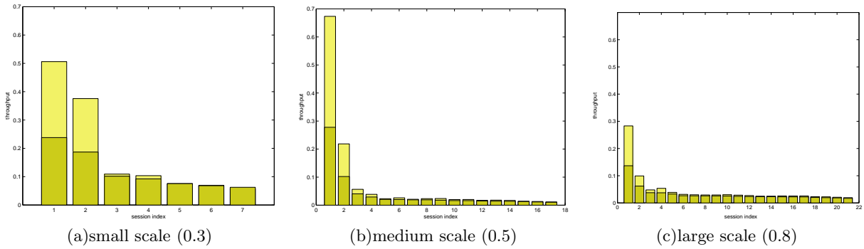
Figure 8: Comparing individual session rate at different density scale networks with (light bar) and without (dark bar) capture ( SINR_{th} of 3.16)
