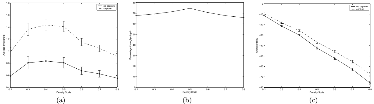
Figure 5: At SINR_{th} = 1 , (a) Network throughput (b) Percentage throughput gain (c) Network utility at different density scales
