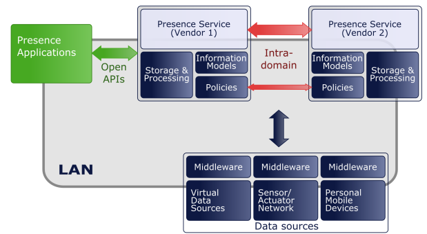
Fig. 4. Intra-domain federation
