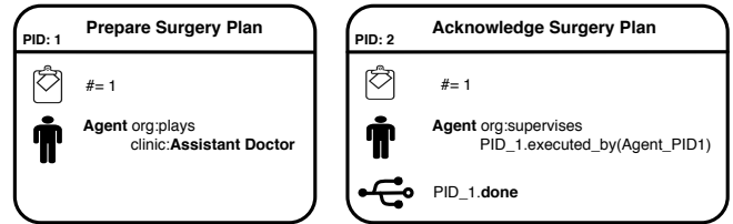
Fig. 3. Clinical example model with organizational dependencies
