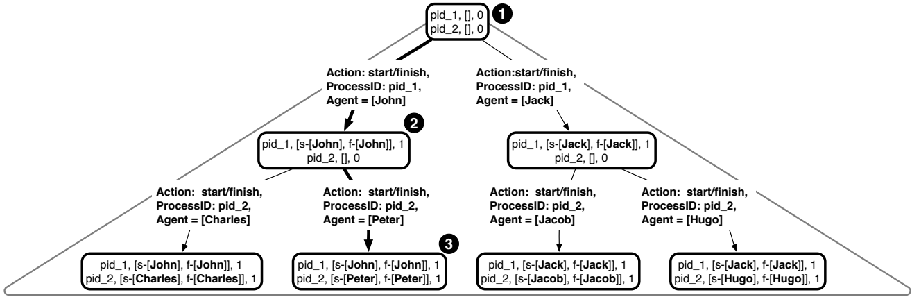
Fig. 5. Illustration of possible execution scenarios of the clinical process model from Figure 3
