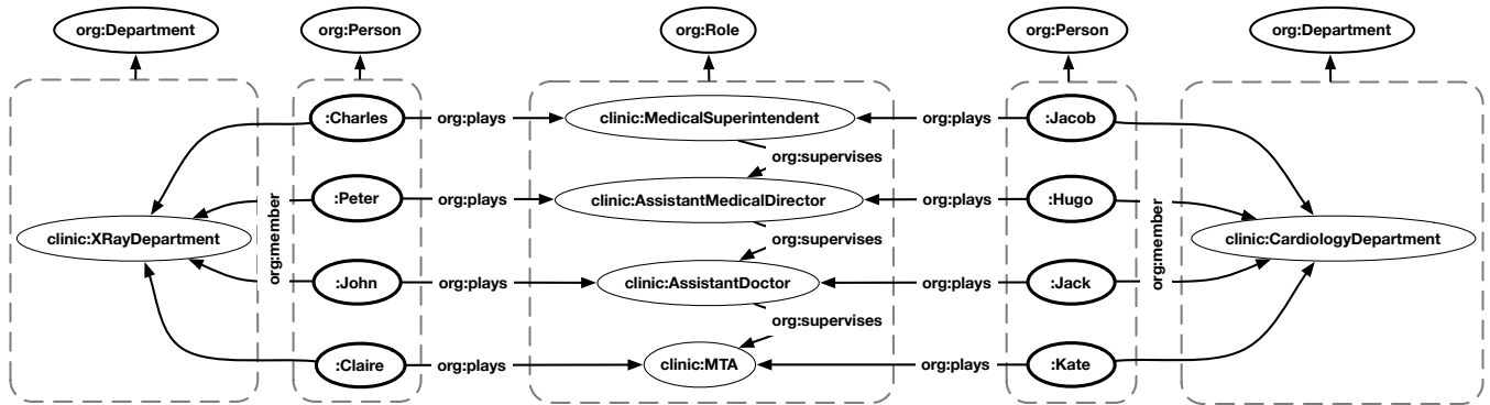
Fig. 4. Extract from a clinical organization representing among others the transitive supervising behavior
