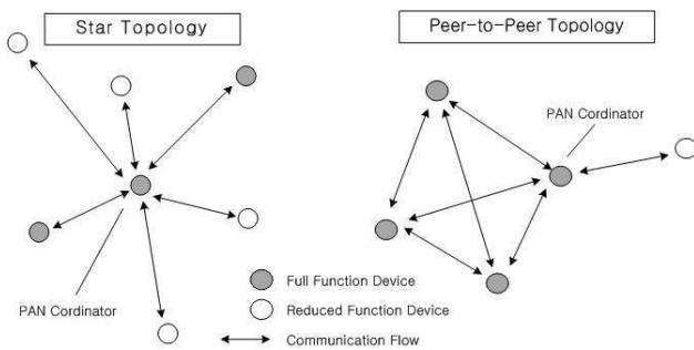
Figure 1. Low Rate WPAN Topology Examples
