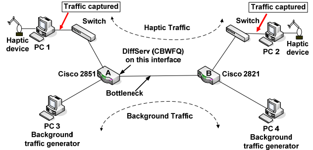
Figure 2. Experimental model of distributed peer-to-peer architecture
