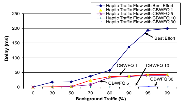
Figure 6. Haptic traffic end-to-end delay versus background with different WFQ weights at egress interface of router A
