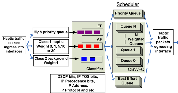
Figure 4. Cisco router Diffserv treatment for haptic and background traffic packets
