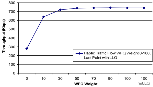
Figure 8. Haptic traffic throughput with different WFQ weights
