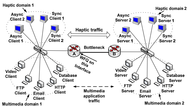
Figure 5. Distributed haptic virtual network simulation model with audio, video, ftp, http and database applications
