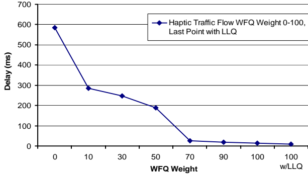
Figure 7. Haptic traffic end-to-end delay with different WFQ weights
