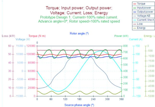
Figure 2. Power-angle curves
