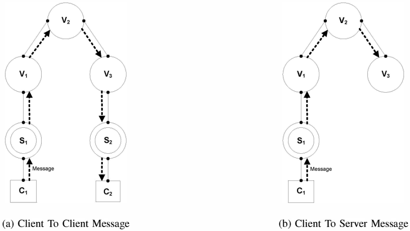
Fig. 3: Clients Interacting With Clients and Objects
