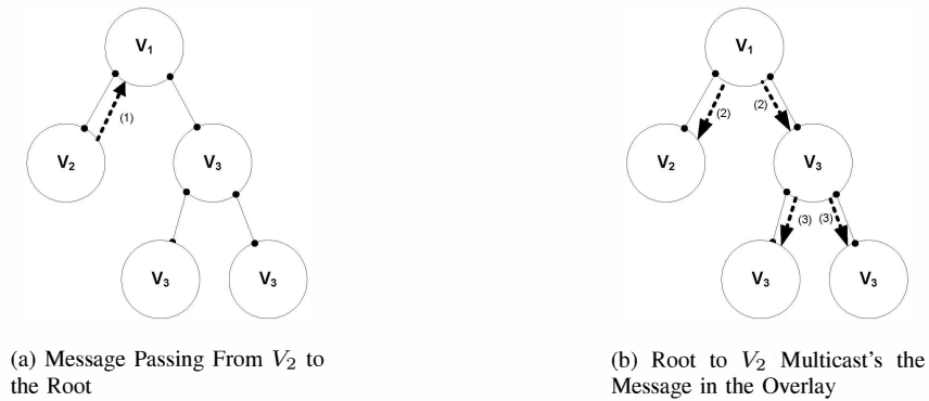
Fig. 4: Message Passing in the Multicast Tree
