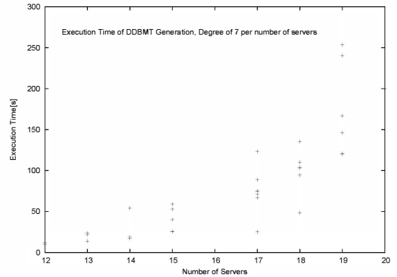
Fig. 9: Number of Nodes vs. Execution Time
