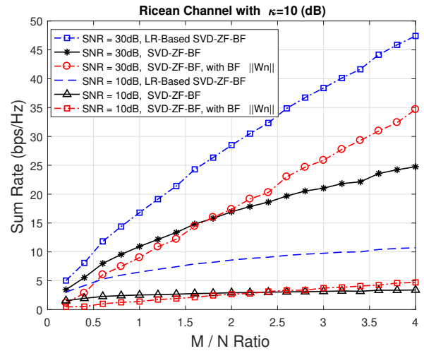
Figure 10. Sum rate versus the 0 < k \leq \frac{M}{N} < \infty , the ratio k is user antennas
