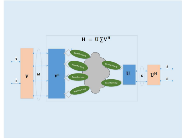
Figure 1. System design with the precoding and beamforming
