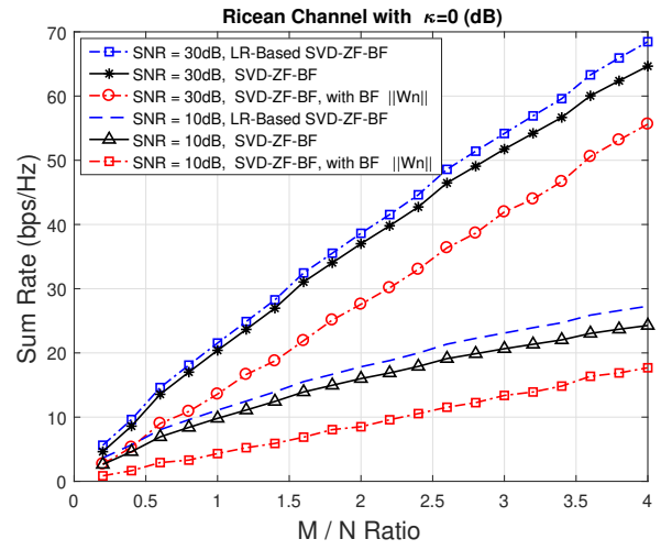
Figure 9. Sum rate versus the 0 < k \leq \frac{M}{N} < \infty , the ratio k is user antenna
