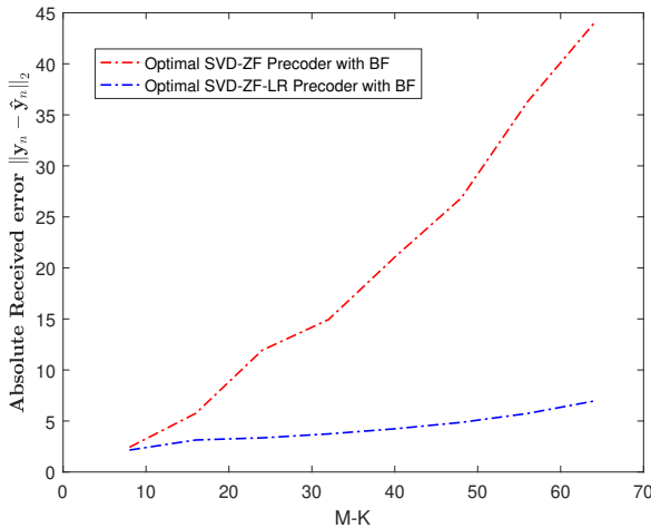
Figure 2. Frobenius norm of the received signals with the (M - K) diversity order
