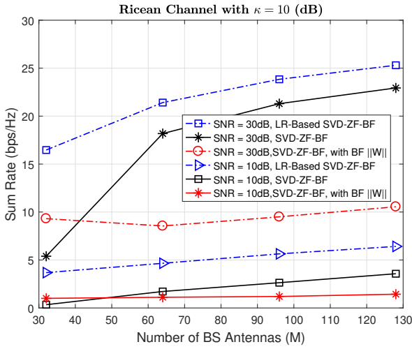
Figure 7. Sum Rate versus the number of BS antenna ( M ), with N users =16 and K = 2
