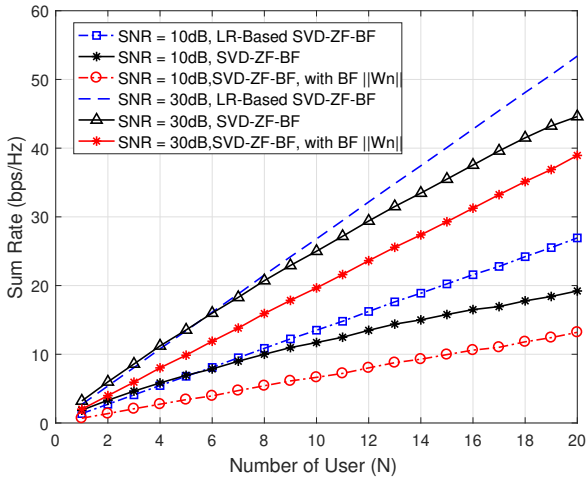
Figure 8. Sum Rate with number of Users ( N ), with M = 128 and K = 2
