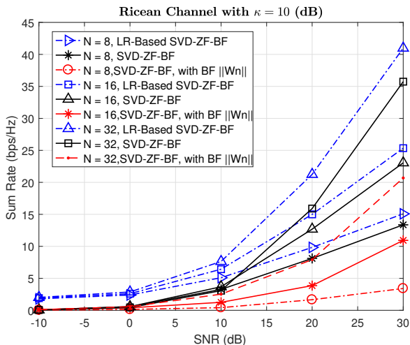
Figure 5. Sum Rate versus the SNR values, with M = 128 and K antennas = 2
