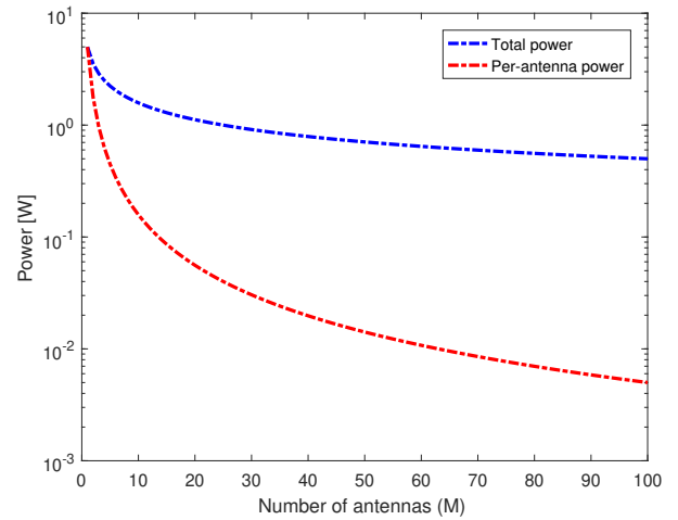
Figure 3. Compares the power utilization of the sum power and per-antenna power allocations
