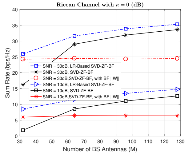
Figure 6. Sum Rate versus the number of BS antenna ( M ), with N users = 16 and K = 2
