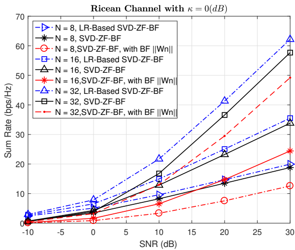
Figure 4. Sum Rate versus the SNR values, with M = 128 and K antennas = 2
