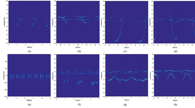
Fig. 1. Spectrograms of eight hand gestures: (a) sliding a hand from right to left, (b) sliding a hand from left to right, (c) pulling, (d) pushing, (e) knocking, (f) moving a hand up and down, (g) waving a hand, (h) patting.
