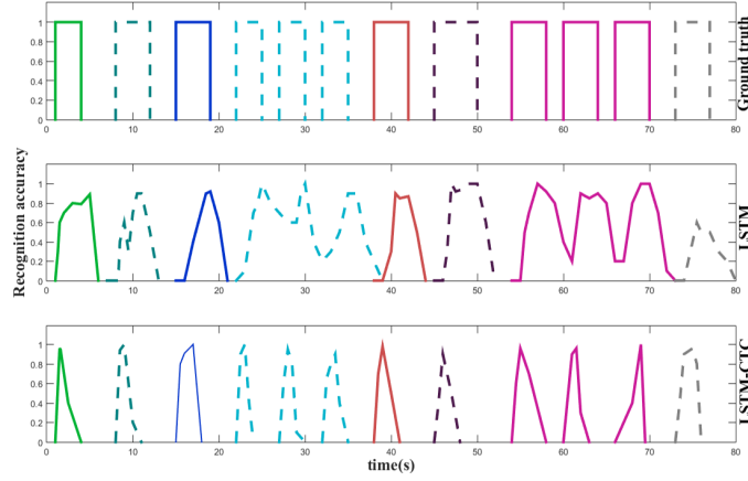
Fig. 2. Comparison of the recognition performance of LSTM and LSTM-CTC.
