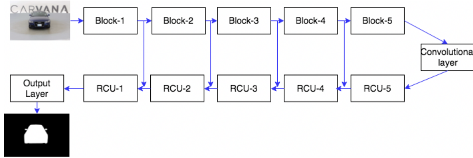
Fig. 5: The overall model architecture.
