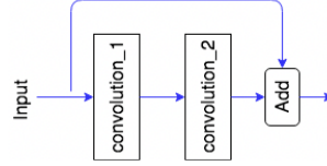
Fig. 4: A residual convolutional unit.
