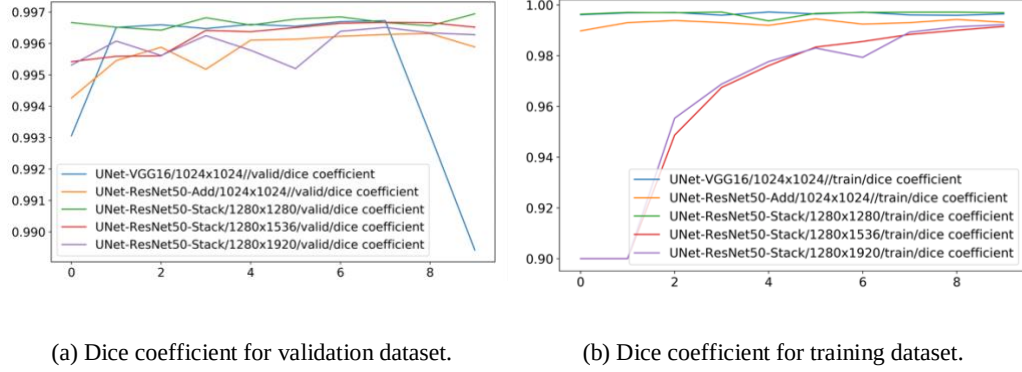
Fig. 7 Dice coefficient of five models.
