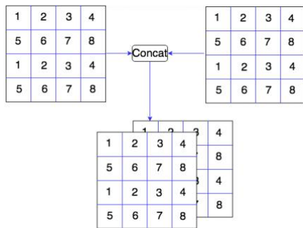
Fig. 2 Example of concat operation on two 1-channel feature maps resulting a two-channel feature map.
