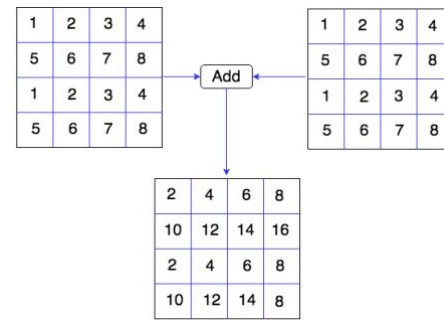
Fig. 3 Example of add operation on two 1-channel feature maps resulting a one-channel feature map which values are addition of the two input feature maps.
