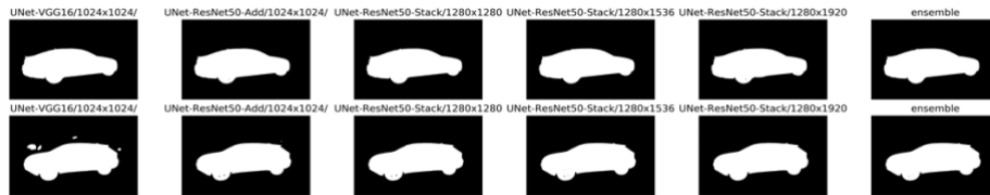
(b) Output segmentation maps of five models and majority voting ensemble.
