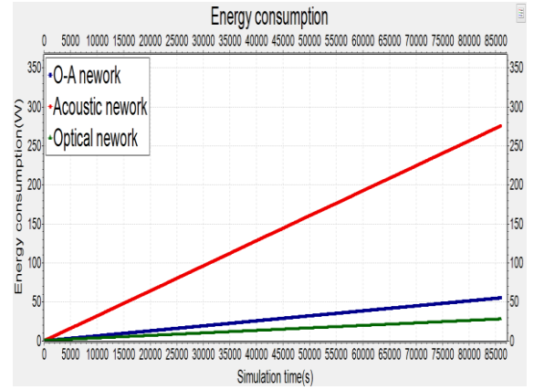
Fig. 5. Energy consumption
