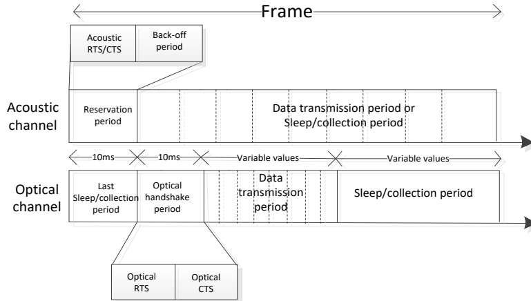
Fig. 2. Frame structure
