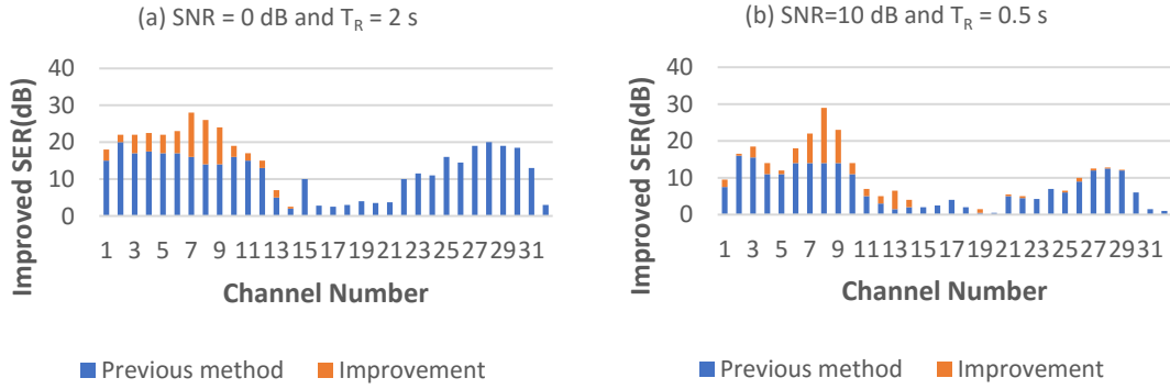
Fig. 1. Improved SER in different noisy reverberant conditions.
