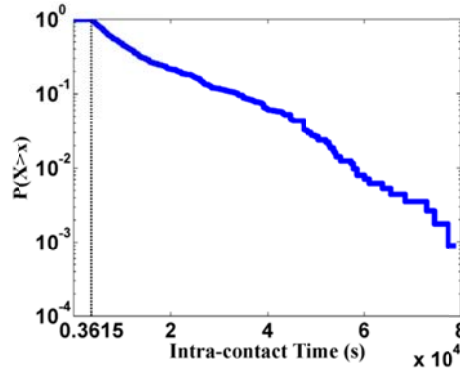
Fig. 2. Intra-contact time CCDF for all users.
