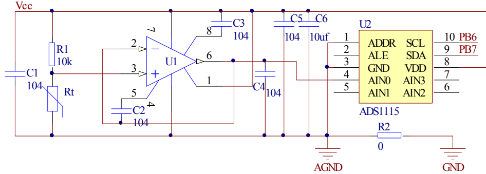
Fig. 3. A/D conversion module circuit diagram
