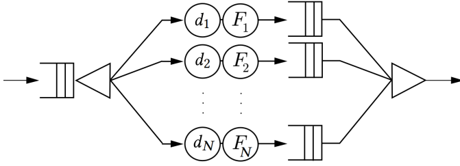
Figure 1: Visualisation of the split-merge system
