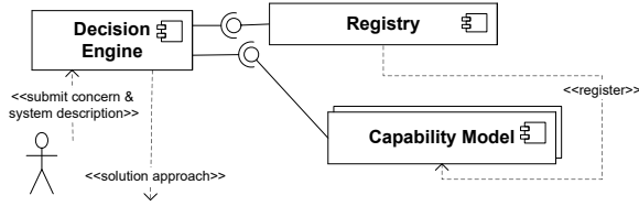
Figure 1: Decision architecture.
