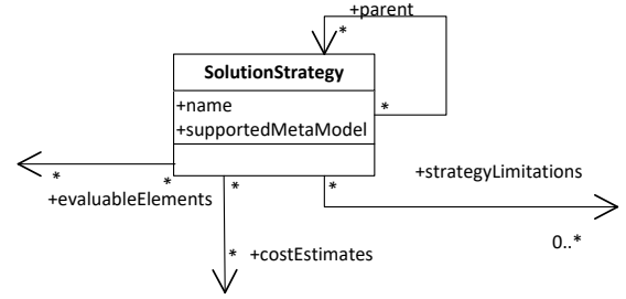
Figure 2: Solution strategy capability model root.
