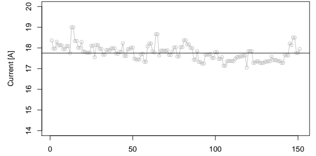
Figure 1: Sample Values over a Short Period of Steady Maneuver Execution (Equidistant Sample Time 100 ms)
