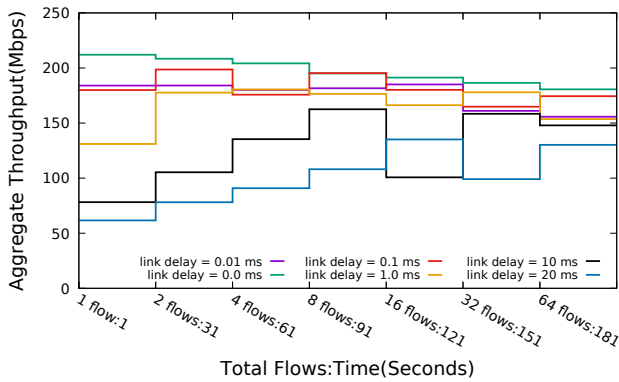
Figure 3: Aggregate throughput by Maxinet.
