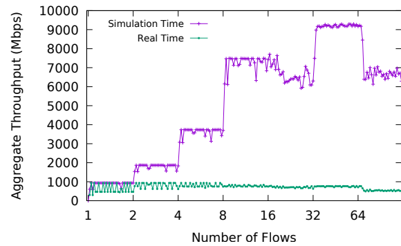
Figure 7: Parallel simulation results.
