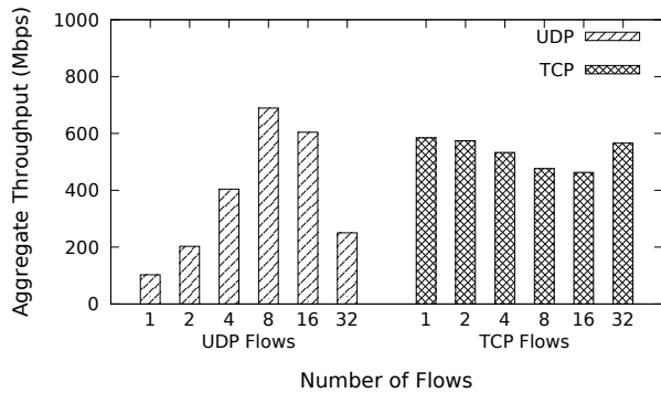
Figure 11: Emulated traffic throughput.
