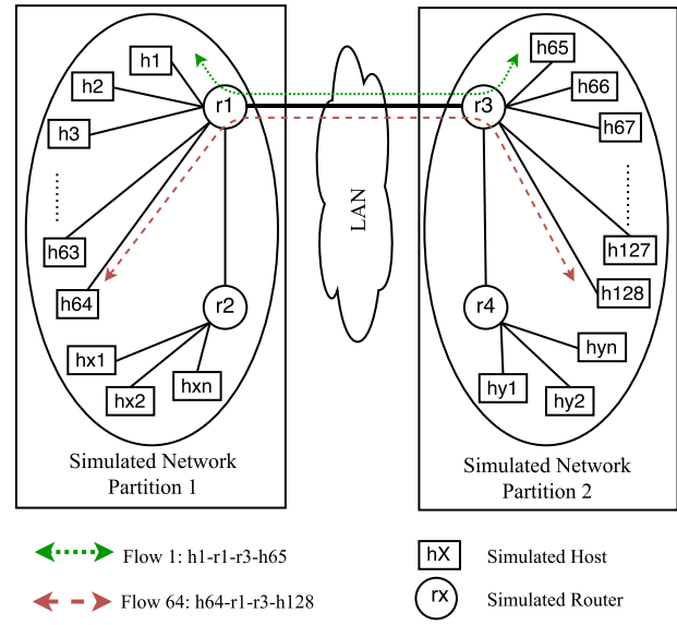
Figure 6: Dumbbell experiment setup.
