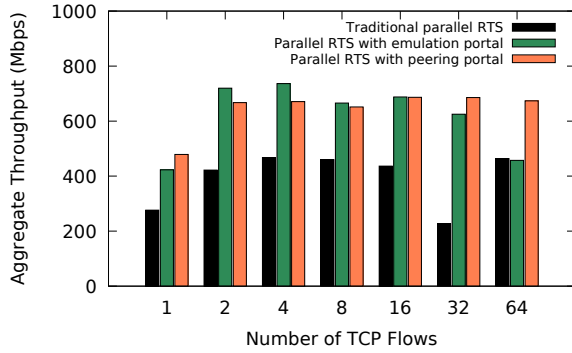
Figure 8: Real-time simulation results.
