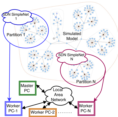
Figure 1: Parallel real-time simulation of a distributed SDN solution on a large hybrid network.
