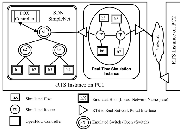
Figure 4: Independent parallel real-time simulation.
