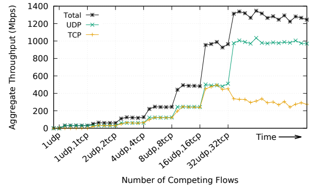
Figure 10: Mixed traffic over peering portals.
