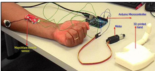
Figure 9. – Overall layout of the system.
