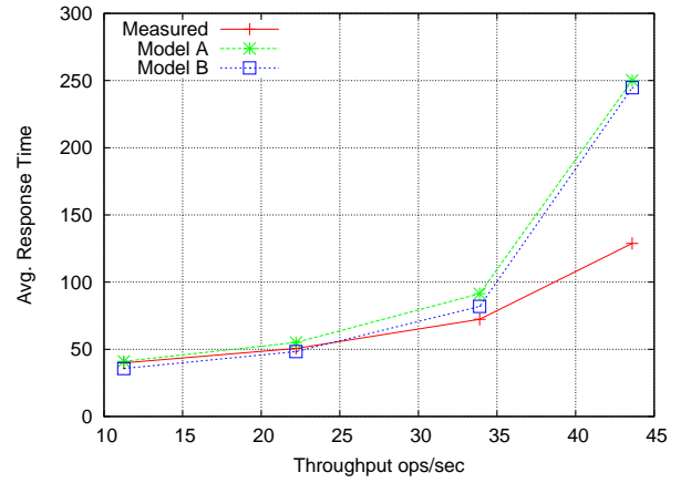
Figure 8: Scenario2a: Validation of the CreateVehicle performance model.
