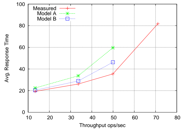
Figure 7: Scenario 1: Validation of the ScheduleWorkOrder performance model.
