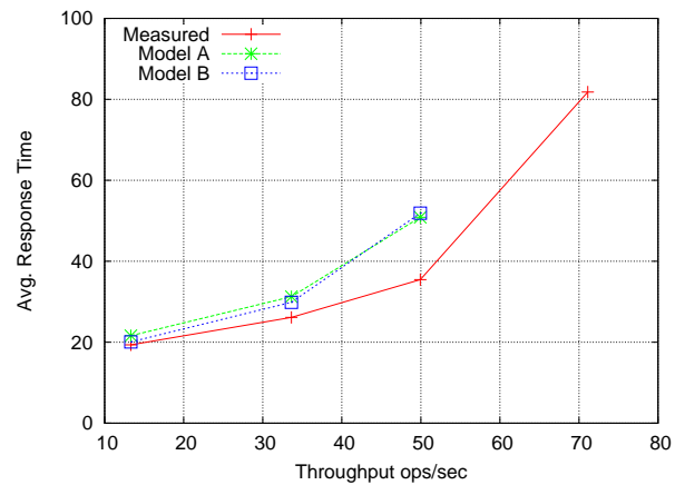
Figure 9: Scenario2b: Validation of the CreateVehicle performance model.
