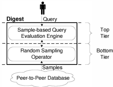
Fig. 2. Two-Tier Architecture of Digest
