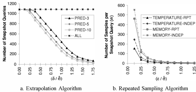
Fig. 4. Effect of the Algorithms
