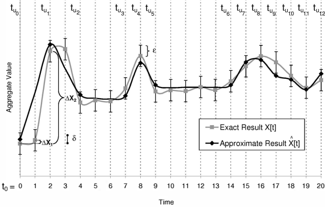
Fig. 1. Fixed-Precision Approximate Continuous Aggregate Query
