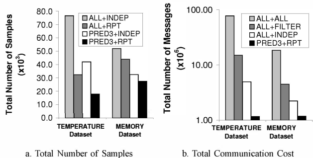
Fig. 5. Efficiency of Digest
