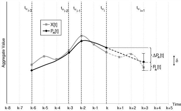
Fig. 3. Computing t_{u_{i+1}} by Polynomial Extrapolation: at t = t_{u_{i+1}} , we have |\Delta P_n[t_{u_{i+1}}]| + |R_n[t_{u_{i+1}}]| > \delta
