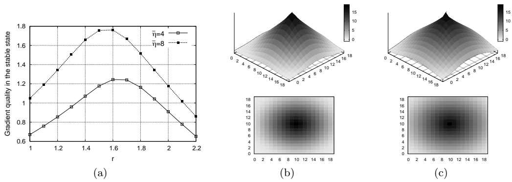
Figure 4: (a) Gradient quality estimator in the stable condition ( \bar{l}_m(\bar{t}) ) with respect to r varying \bar{n} . (b) Pheromone gradient over \mathcal{V} when r = r^* = 1.6 ( \bar{n} = 4 ). (c) Pheromone gradient over \mathcal{V} when r = r^* = 1.6 ( \bar{n} = 8 ).
