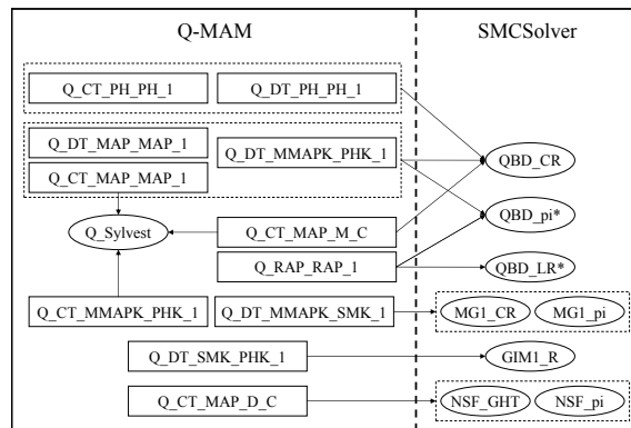
Figure 1: Dependency Graph of the Q-MAM Tool
