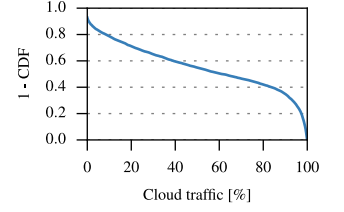
Figure 9: Cloud traffic produced by mobile websites.
