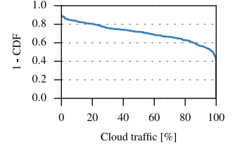
Figure 5: Cloud traffic produced by individual apps.
