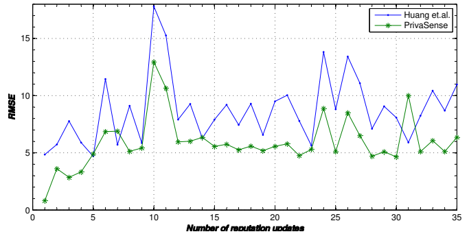
Figure 5: The effect of cloaked reputation scores in different systems
