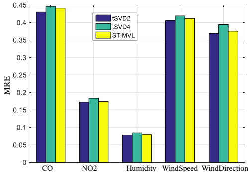
Figure 6: Comparing our method with ST-MVL on five meteorological datasets in terms of MRE
