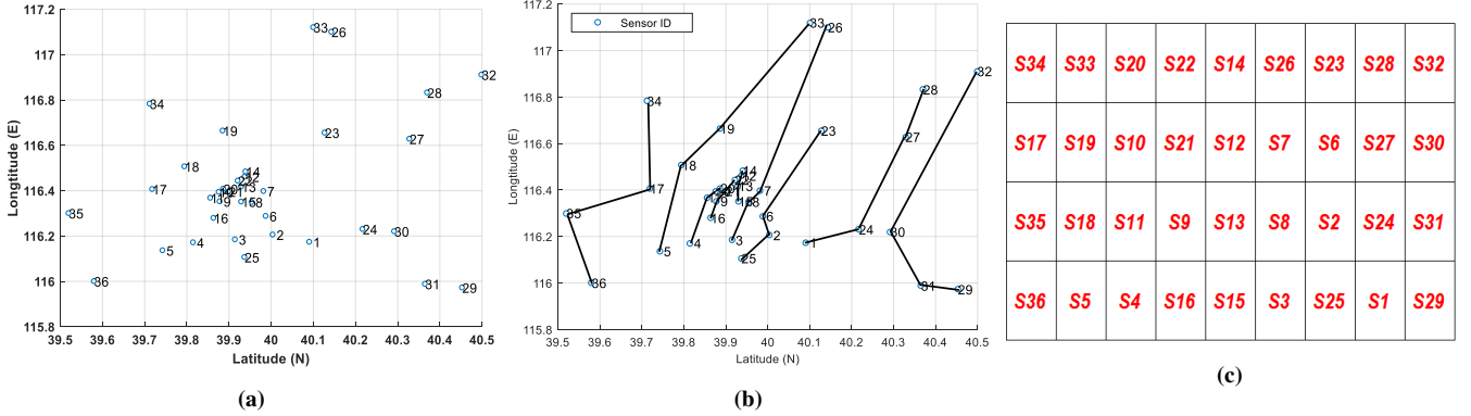
Figure 3: (a) The spatial locations of PM2.5 sensor stations throughout the city; (b) The searching result by using NN-based heuristic searching method; (c) The mapped matrix of sensor array
