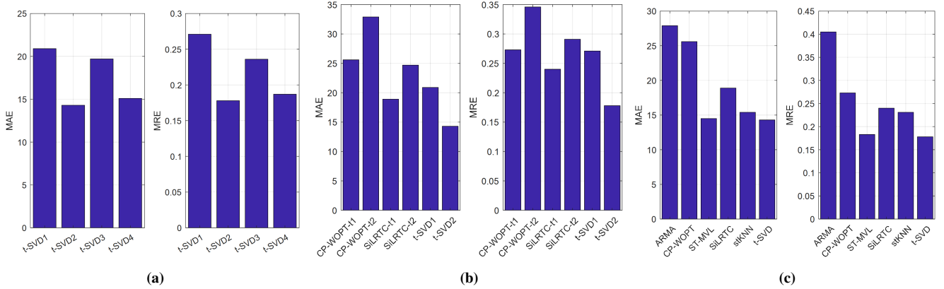
Figure 4: (a) Recovery accuracies for different tensor formulations; (b) Comparison of recovery accuracies for different tensor-based methods; (c) Comparison of state-of-the-art sensor reading recovery methods
