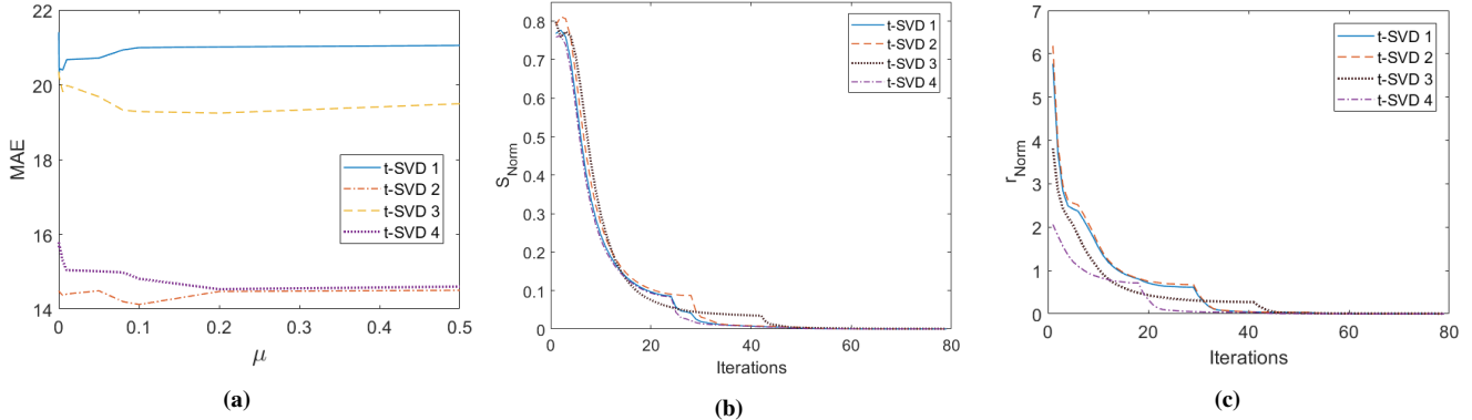
Figure 5: (a) Impact of parameter \mu to the recovery accuracy; (b) Convergence of our model in terms of s_{Norm} ; (c) Convergence of our model in terms of r_{Norm} ;
