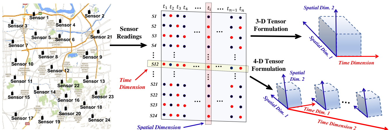
Figure 1: The idea of tensor formulation: Many tensors are irregularly deployed throughout the city (shown by the first figure), and they generate huge amount of time series data that normally have two dimensions - time and spatial dimensions (shown by the second figure). Those sensor readings are easily missing or lost (represented by the red dots), so this paper aims to recover those missing sensor readings. The idea is to formulate the data as a 3-order tensor such as two spatial dimensions (i.e., longitude and latitude) plus one time dimension, or 4-order tensor such as two spatial dimensions and two time dimensions (e.g., hours \times days).
