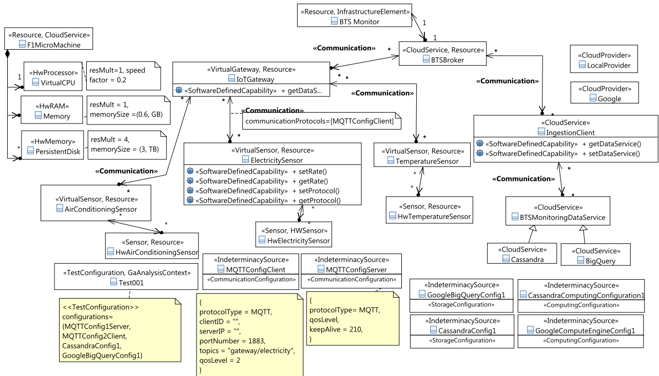
Figure 6: Annotated Class Diagram of the Telco BTS monitoring system showing structure and test configuration.
