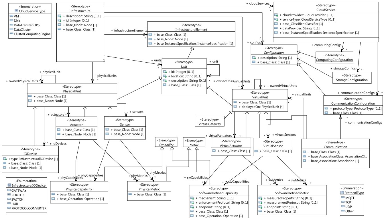
Figure 2: Infrastructure profile: excerpt of stereotypes and their relationships.
