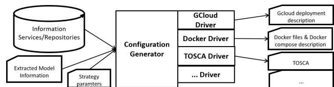
Figure 5: Deployment configuration and description generator
