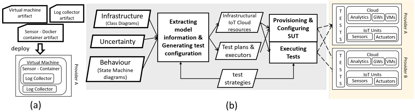
Figure 1: (a) Artifacts and their deployment, (ii) Tool pipeline for dynamic SUT provisioning
