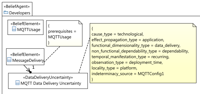
Figure 7: Data uncertainty modeling affecting the TemperatureSensor behavior modeled as UML StateMachine.
