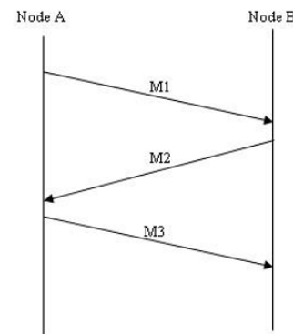
Fig. 5. Authentication Protocol [3]
