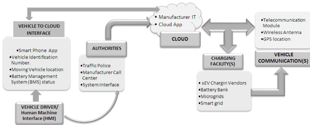
Fig. 5: Federated V2C framework for smart charging of xEVs.
