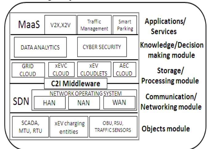
Fig.4: Service Oriented Architecture (SOA) for TOSCs
