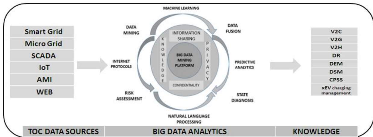
Fig. 7: Workflow model for Big-Data processing in TOSC Architectures
