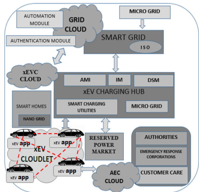
Fig. 3: Architecture of the Cloud aware Transport Oriented Smart City
