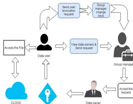
Figure 2. CP-ABE
