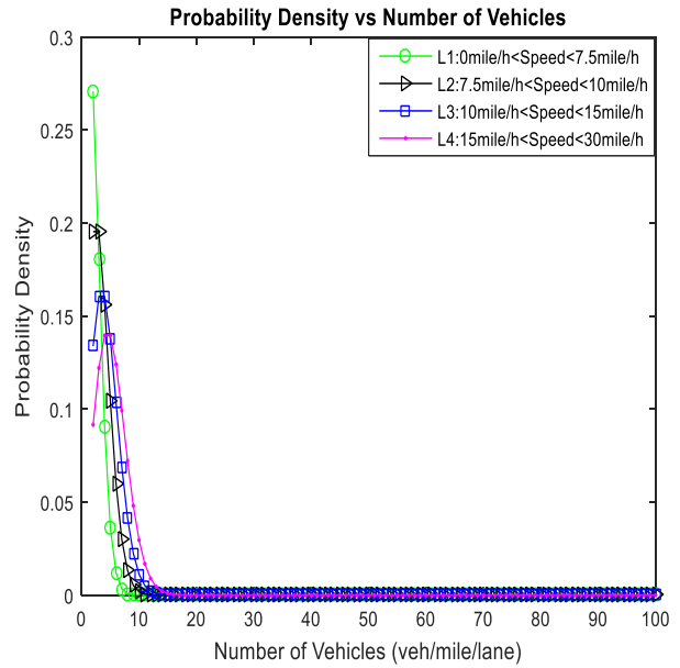
Figure 4. The effect of traffic flow when \lambda = 2
