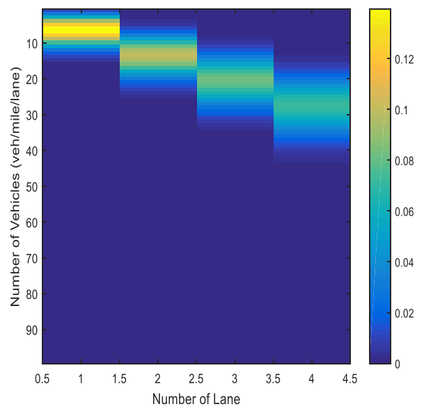
(h). \lambda = 8
