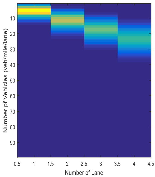
(g). \lambda = 7
