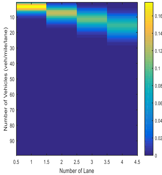
(e). \lambda = 5
