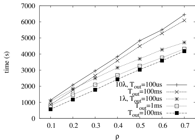
Figure 10: Processing time of OBS scenario with 1 and 10 wavelength and different timer vs load in the central link
