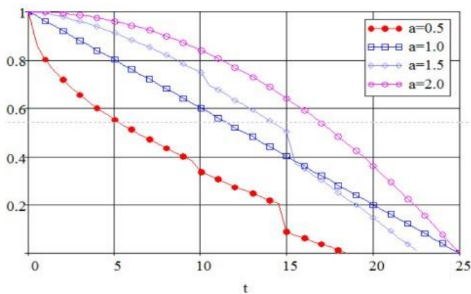
Figure 7. Functions of resistance to refusal by formation of defects and their partial elimination
