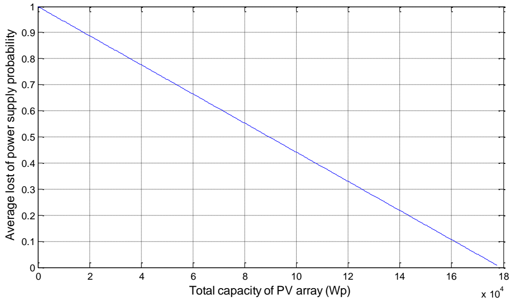
Figure 8. Variation of total PV capacity versus average loss of power supply probability
