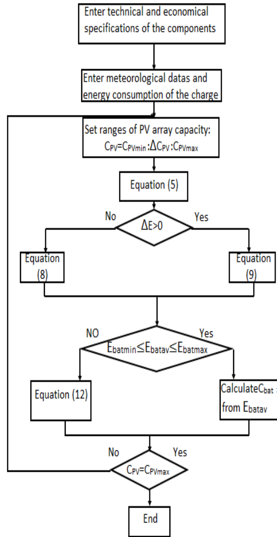
Figure 5. Calculation of the system storage capacity method
