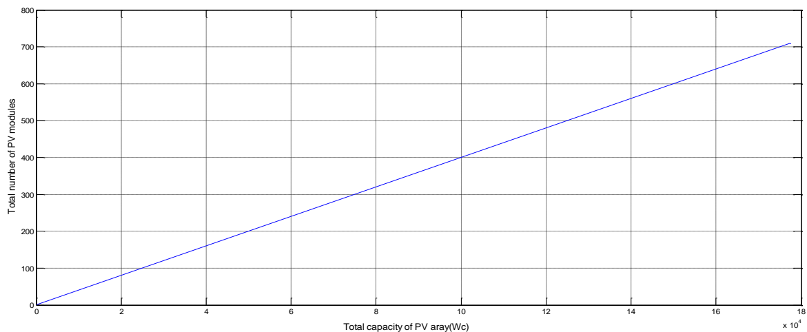
Figure 6. Variation of total PV number versus total PV capacity obtained with the intuitive method
