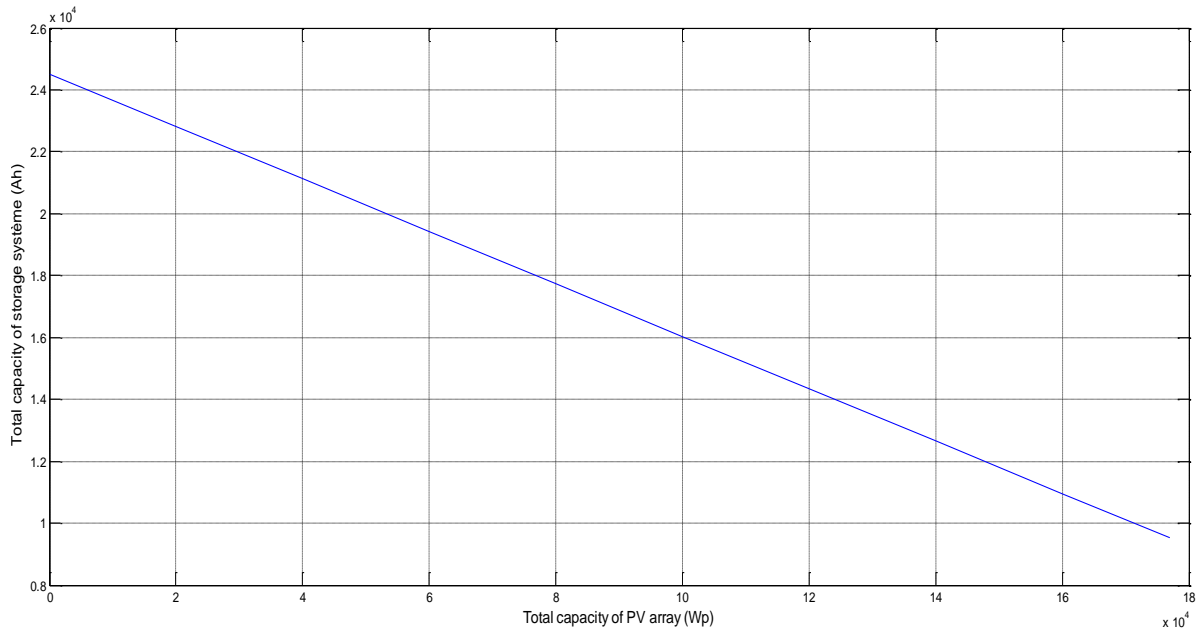
Figure 11. Different PV/battery combinations at ALPSP of 0.01
