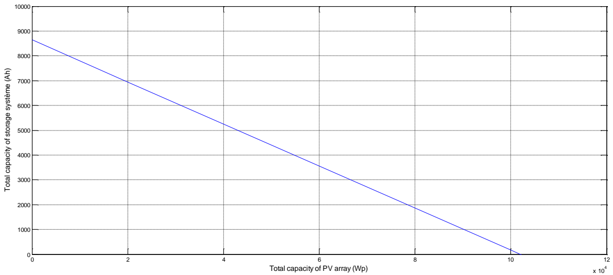
Figure 10. Different PV/battery combinations at ALPSP of 1
