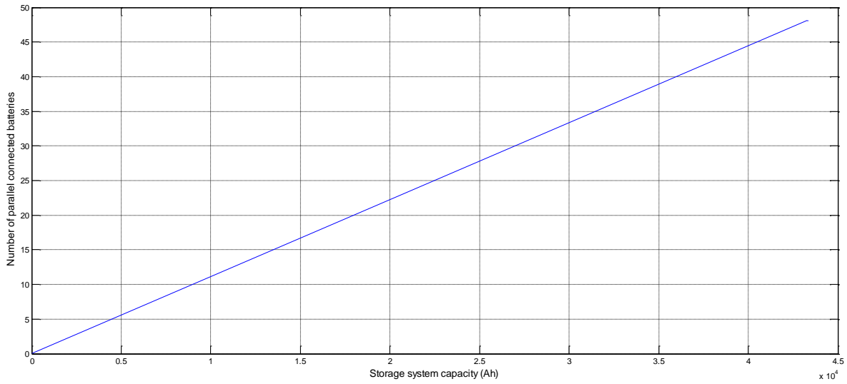
Figure 7. Variation of number of parallel connected batteries versus total storage system capacity obtained with intuitive method
