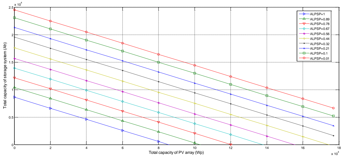
Figure 9. Different PV/battery combinations versus different values of average loss of power supply probability
