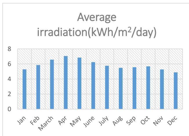
Figure 1. Annual variation of monthly average irradiation of Ngoundiane Site
