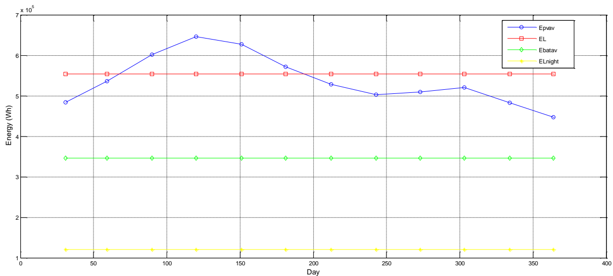
Figure 12. Annual variation of PV average output ( E_{PVav} ), maximal load demand ( E_L ), average energy supplied by batteries ( E_{batav} ), and maximal load demand during night ( E_{Lnight} )
