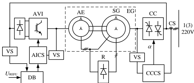
Figure 2. Functional diagram of stabilizing system of the electrical output voltage parameters by means of AC excitation winding circuit
