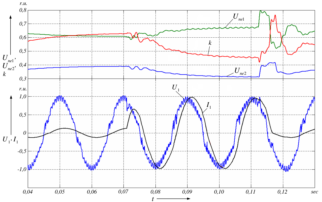
Figure 11. Load voltage and current waveforms of MCS when changing load power while stabilizing output electrical parameters of MCS by means of AC excitation winding circuit
