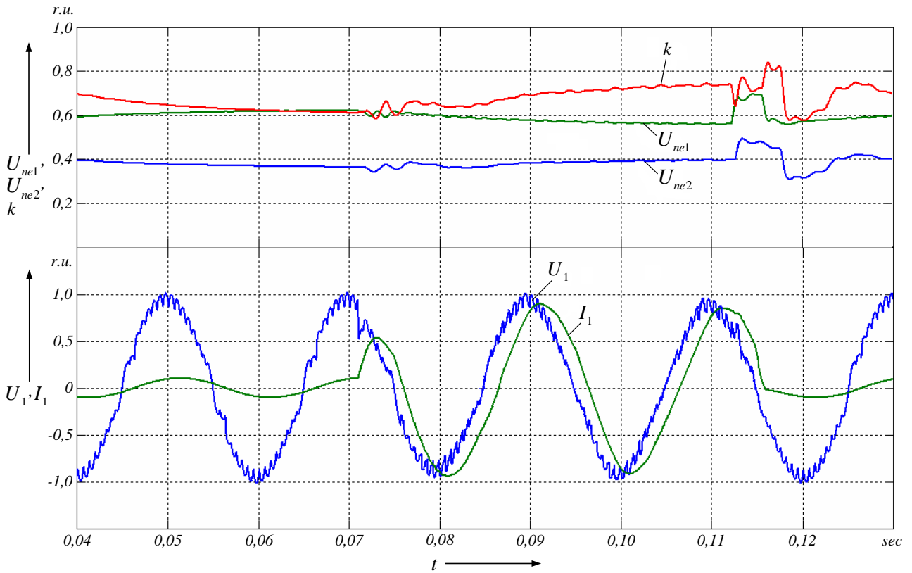
Figure 9. Load voltage and current waveforms of MCS when changing load power while stabilizing output electrical parameters of MCS by means of DC excitation winding circuit
