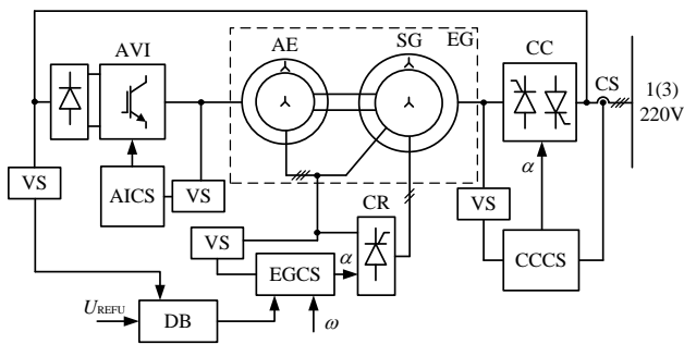
Figure 1. Functional diagram of stabilizing system of the electrical output voltage parameters by means of DC excitation winding circuit
