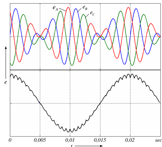
Figure 4. EMF waveforms of armature windings of generator and the output voltage envelope of MCS
