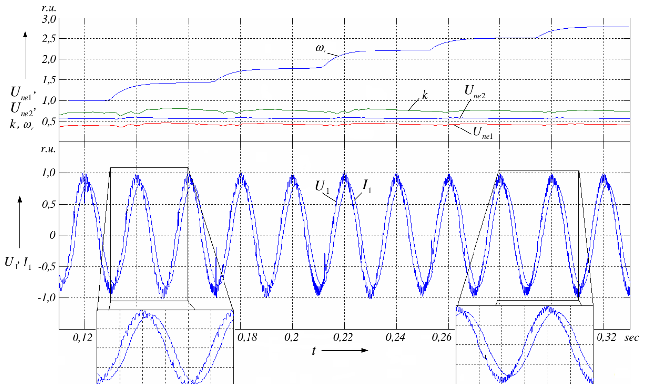
Figure 11. Load voltage and current waveforms of MCS when changing load power while stabilizing output electrical parameters of MCS by means of AC excitation winding circuit
