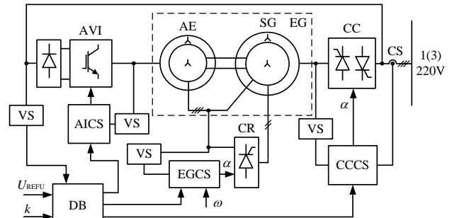
Figure 3. Functional diagram of stabilizing system of the electrical output voltage parameters of combined type
