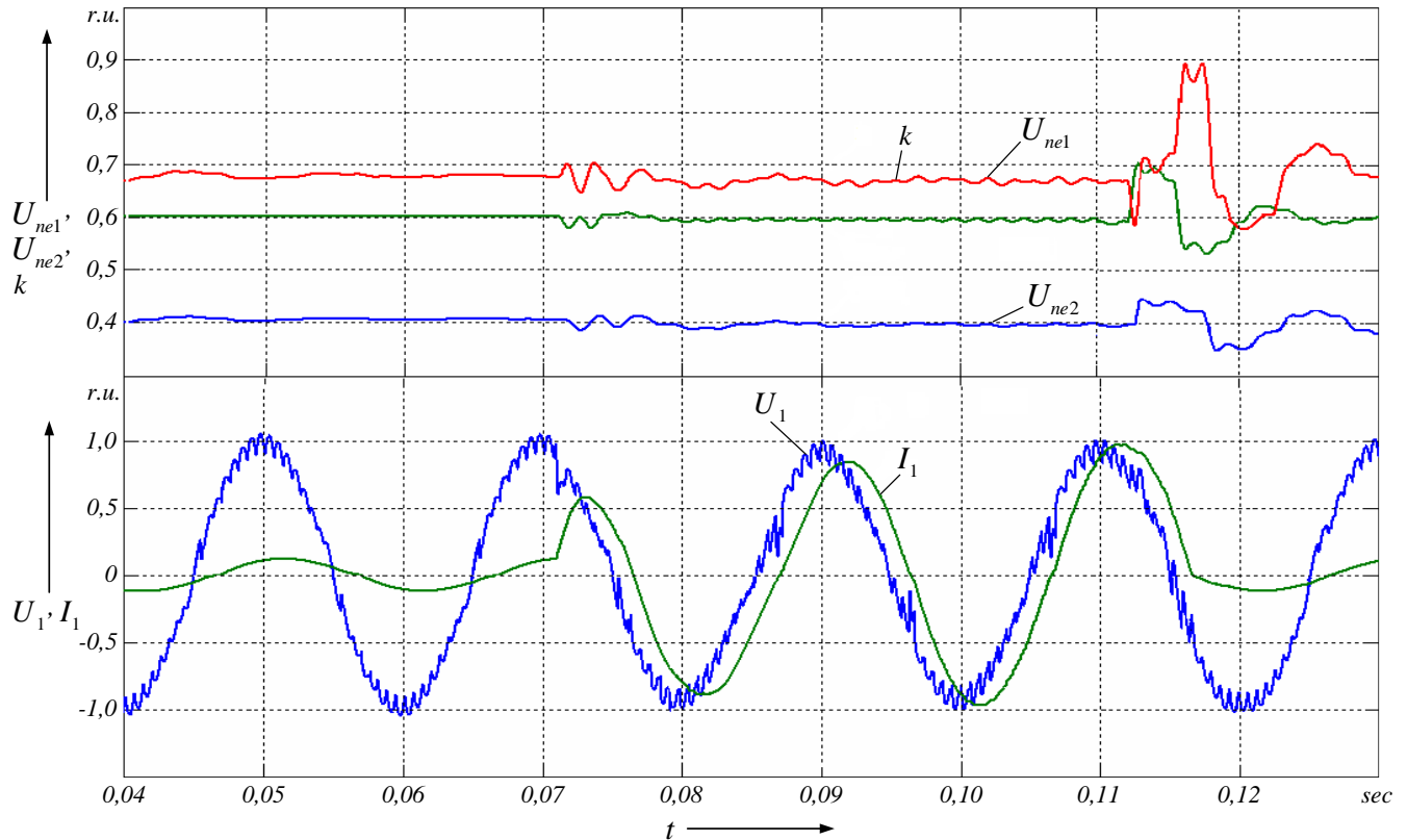
Figure 13. Load voltage and current waveforms of MCS when changing load power while stabilizing output electrical parameters of MCS by means of DC and AC excitation winding circuit
