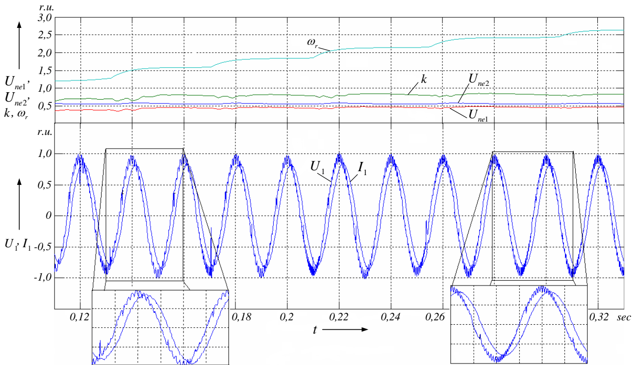
Figure 10. Load voltage and current waveforms of MCS when changing rotational speed of driving shaft while stabilizing output electrical parameters of MCS by means of AC excitation winding circuit
