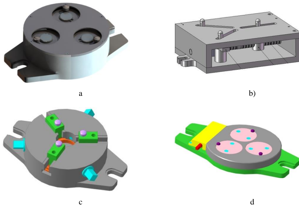
Figure 1. Adjustable locating modules for setup of prismatic parts according to the plane
