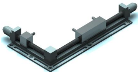
Figure 2. Adjustable locating module for locating of prismatic parts in “quadrantal angle”
