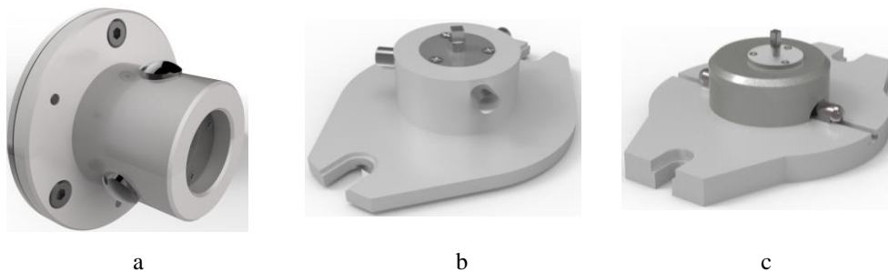
Figure 4. Adjustable locating modules for locating of parts according to internal cylindrical surfaces
