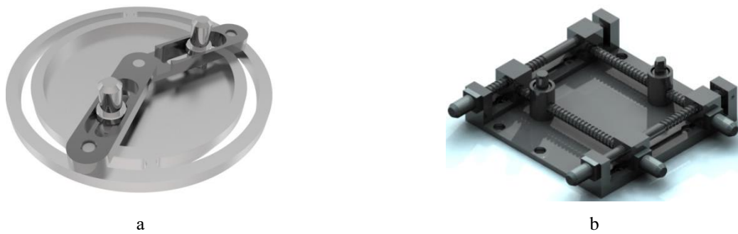
Figure 3. Adjustable locating modules for locating of prismatic parts according to plane and two holes
