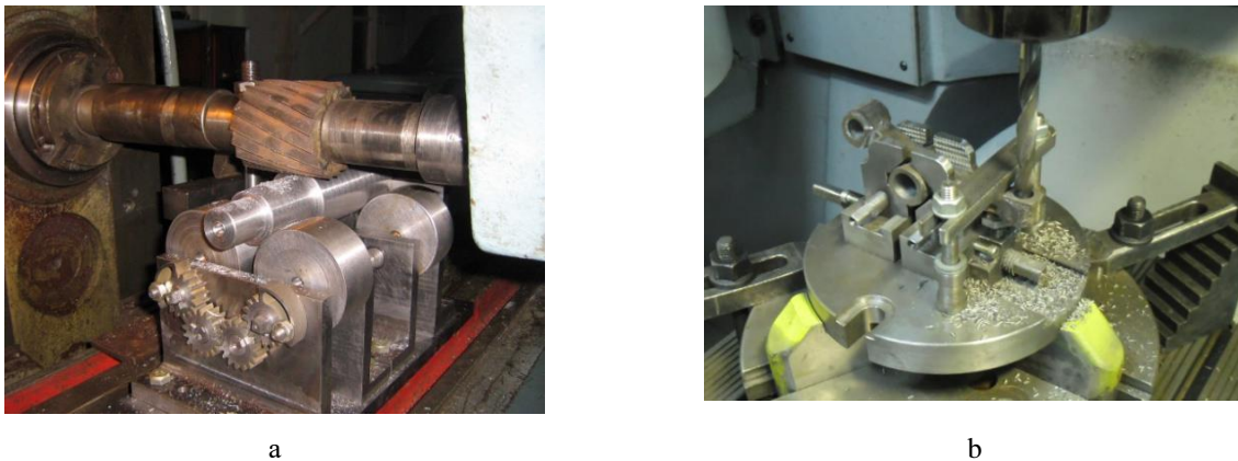
Figure 6. Experimental researches of modular adjustable fixtures for shafts (a) and levers (b)
