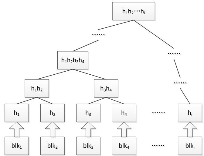
Figure 3. The storage structure that can be used by a prover to reduce its computational complexity when generating proofs. Each leaf h_i stores the hash value of a block, and each internal node stores the product of the values stored at its two children.
