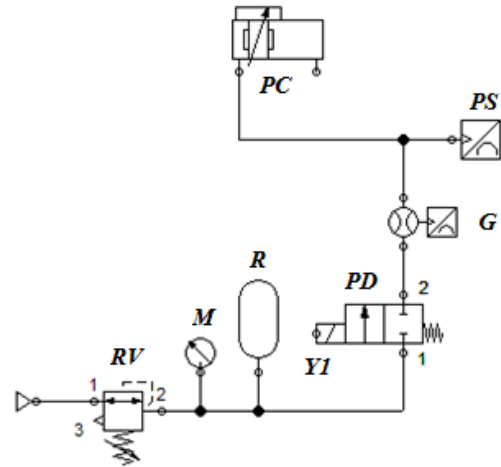
Figure 2. Principle pneumatic diagram of the research stand for measuring the "dead" volume
