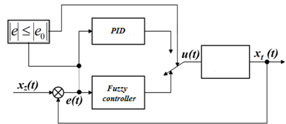
Figure 7. Diagram of a hybrid control algorithm for a carriage of rodless pneumatic actuator based on fuzzy logic and a PID controller
