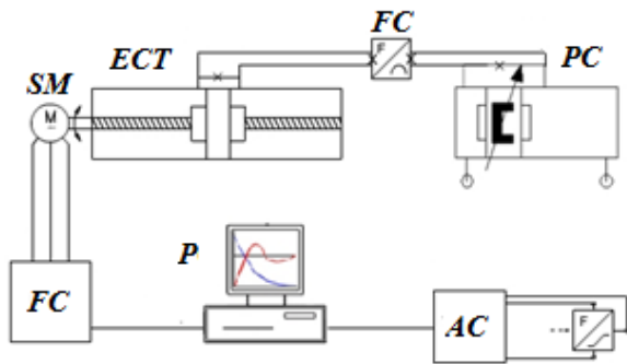
Figure 3. Structural diagram of the friction force test stand in a rodless pneumatic cylinder
