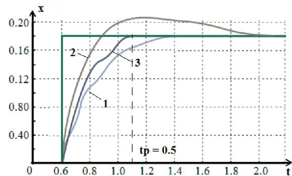
Figure 8. The transient process of positioning error when the regulator is operated on the basis of fuzzy logic (1), PID controller (2), and hybrid algorithm (3).
