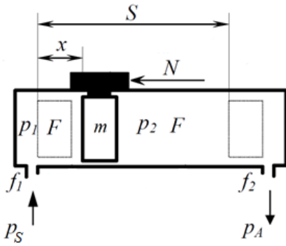
Figure 1. Rodless pneumatic actuator circuit scheme
