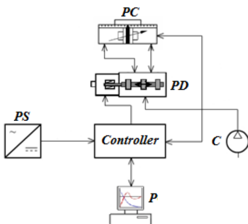
Figure 4. Structural diagram of the rodless pneumatic drive positioning system
