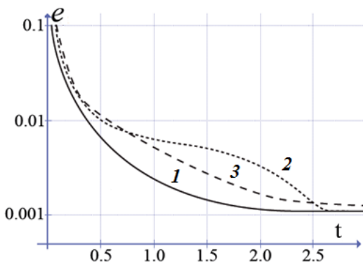
Figure 6. Dependence of the accuracy of the fuzzy controller on the defuzzification method: 1) the center of gravity method, 2) the median method, 3) the maximum method
