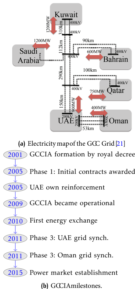
Figure 12. GCC interconnecting grid overview
