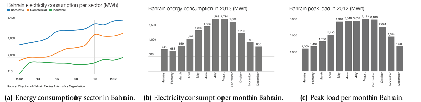
Figure 7. Bahrain Power Grid Statistics
