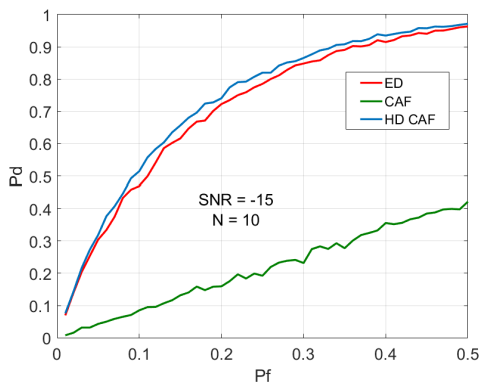
Figure 9. The ROC curves for HD CAF (without uncertainty of spectral density of noise power estimation influence)
