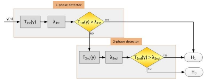
Figure 1. Scheme of the hybrid detector
