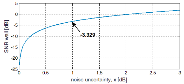
Figure 3. ‘SNR Wall’ in a noise uncertainty function
