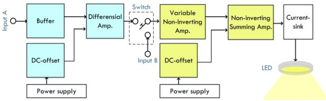
Fig. 2. Block diagram of proposed LED driver circuit for communication and illumination
