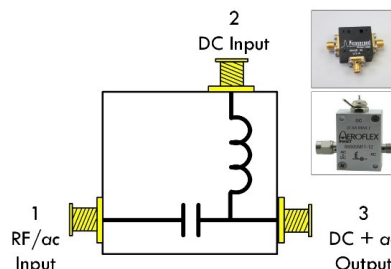
Fig. 1. Basic configuration of commercial bias-T which is consist of inductor & capacitor component, and real product Aeroflex® that retrieved from Apitech.corp. [14].
