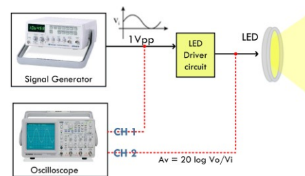
Fig. 6. Test scenario to observe cut-off frequency of the LED driver, testing is done using sinusoidal input signal and output gain voltage calculated using equation 20 * \log (V_o/V_i)
