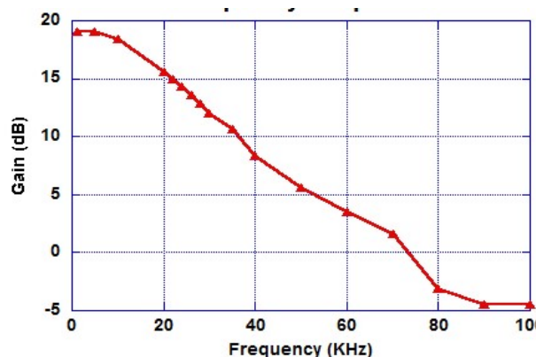
Fig. 11. LED driver bandwidth, frequency is ranging from 1 kHz to 100 kHz
