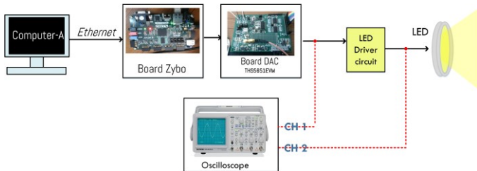
Fig. 7. Set-up of the second scenario
