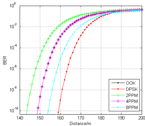
Figure 4. BER versus distance
