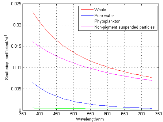
Figure 2. Scattering spectra of seawater
